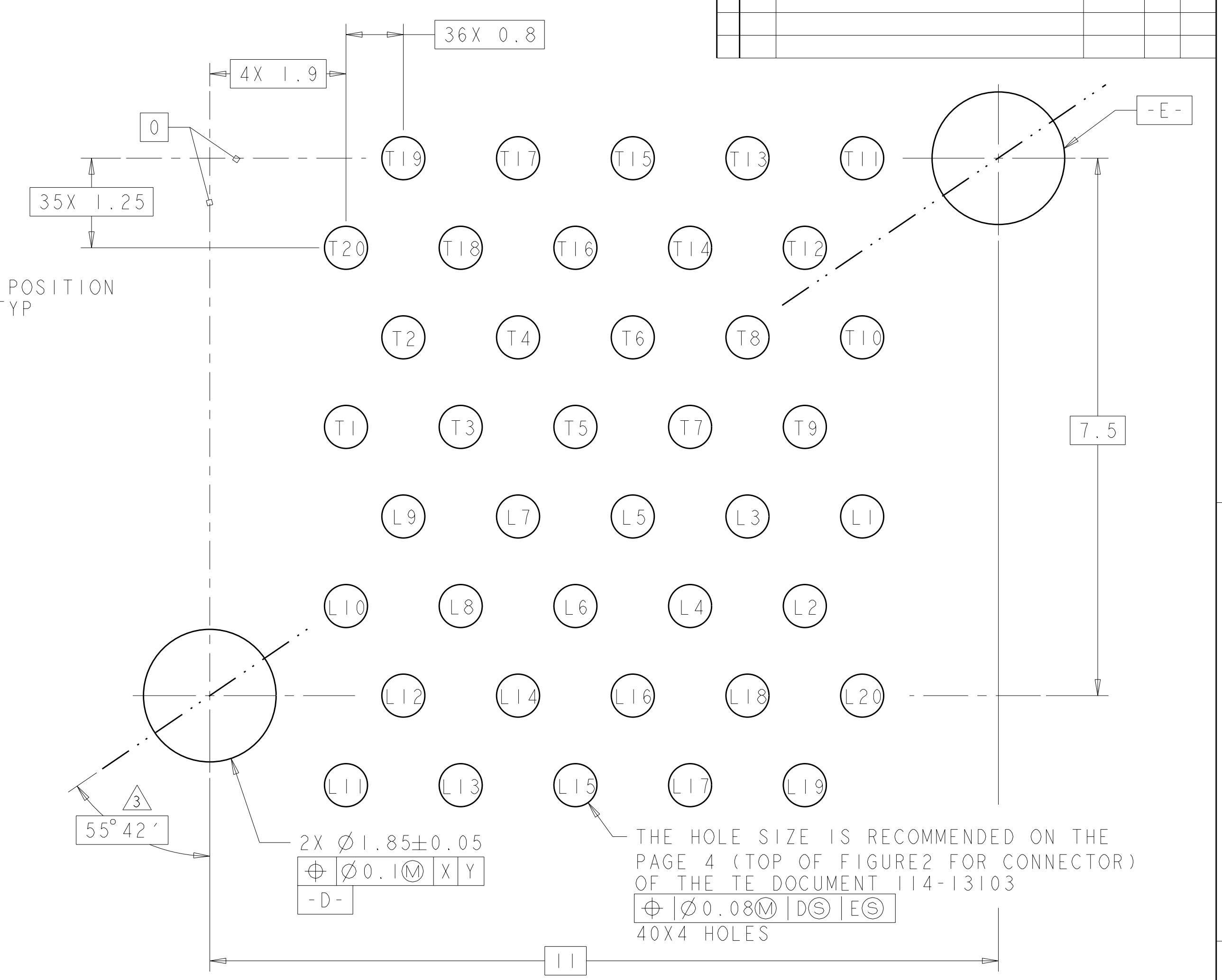
DETAIL G RECOMMENDED PT CONNECTOR CONFIGURATION 4X INDIVIDUALLY SCALE 20:1
