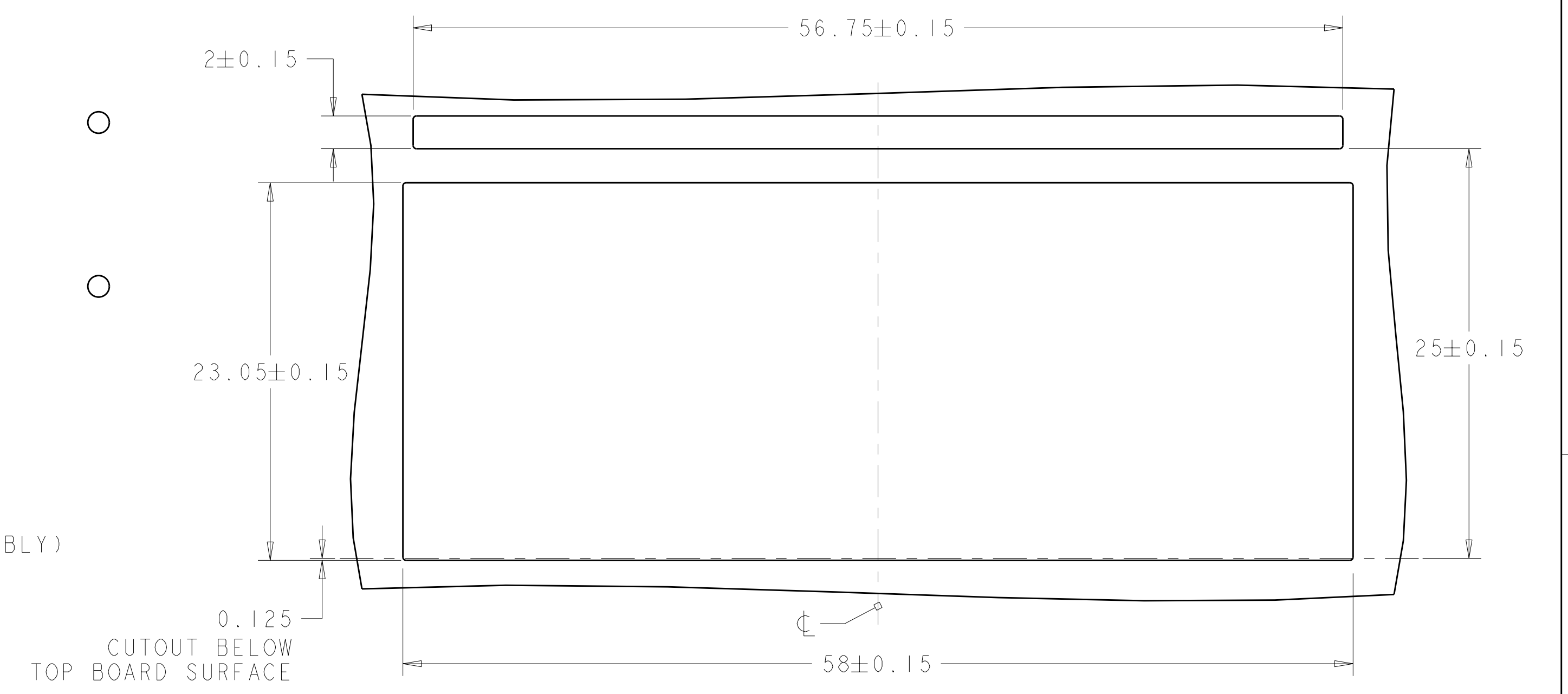
RECOMMENDED BEZEL CUTOUT SCALE 4:1
